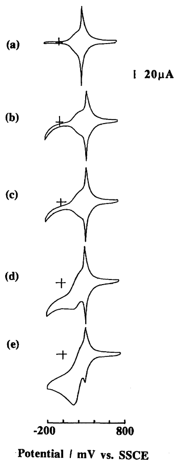
Fig. 5. Cyclic voltammograms of the gold electrode modified with \text{FcC}_{11}\text{SH} by dipping treatment in 1 mM \text{FcC}_{11}\text{SH} hexane solution for 50 h. Solution: (a) 1 M \text{HClO}_4 , (b) 1 mM \text{Fe}^{\text{III}}(\text{edta})/0.1 M \text{HClO}_4 , (c) 1 mM \text{Fe}^{\text{III}}(\text{edta})/0.2 M \text{HClO}_4 , (d) 1 mM \text{Fe}^{\text{III}}(\text{edta})/0.5 M \text{HClO}_4 , and (e) 1 mM \text{Fe}^{\text{III}}(\text{edta})/1 M \text{HClO}_4 . Sweep rate: 100 \text{ mV s}^{-1} .
