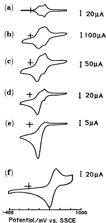
Fig. 1. Cyclic voltammogram of a gold electrode, which was dip-treated in 1 mM FeC_{11}SH hexane solution for 96 h (a) measured in 1 M HClO_4 with sweep rate of 100 mV s^{-1} and (b)–(e) measured in a solution containing 1 M HClO_4 and 1 mM Fe(ClO_4)_3 with sweep rate of (b) 1000 mV s^{-1} , (c) 500 mV s^{-1} , (d) 100 mV s^{-1} , and (e) 10 mV s^{-1} . Cyclic voltammogram of an untreated gold electrode measured in a solution containing 1 M HClO_4 and 1 mM Fe(ClO_4)_3 with a sweep rate of 100 mV s^{-1} is presented as a comparison (f).
